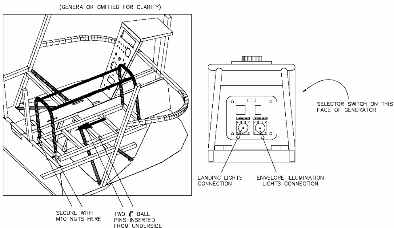
FIG. 10.2.2. INSTALLATION OF NIGHT LIGHTING GENERATOR
